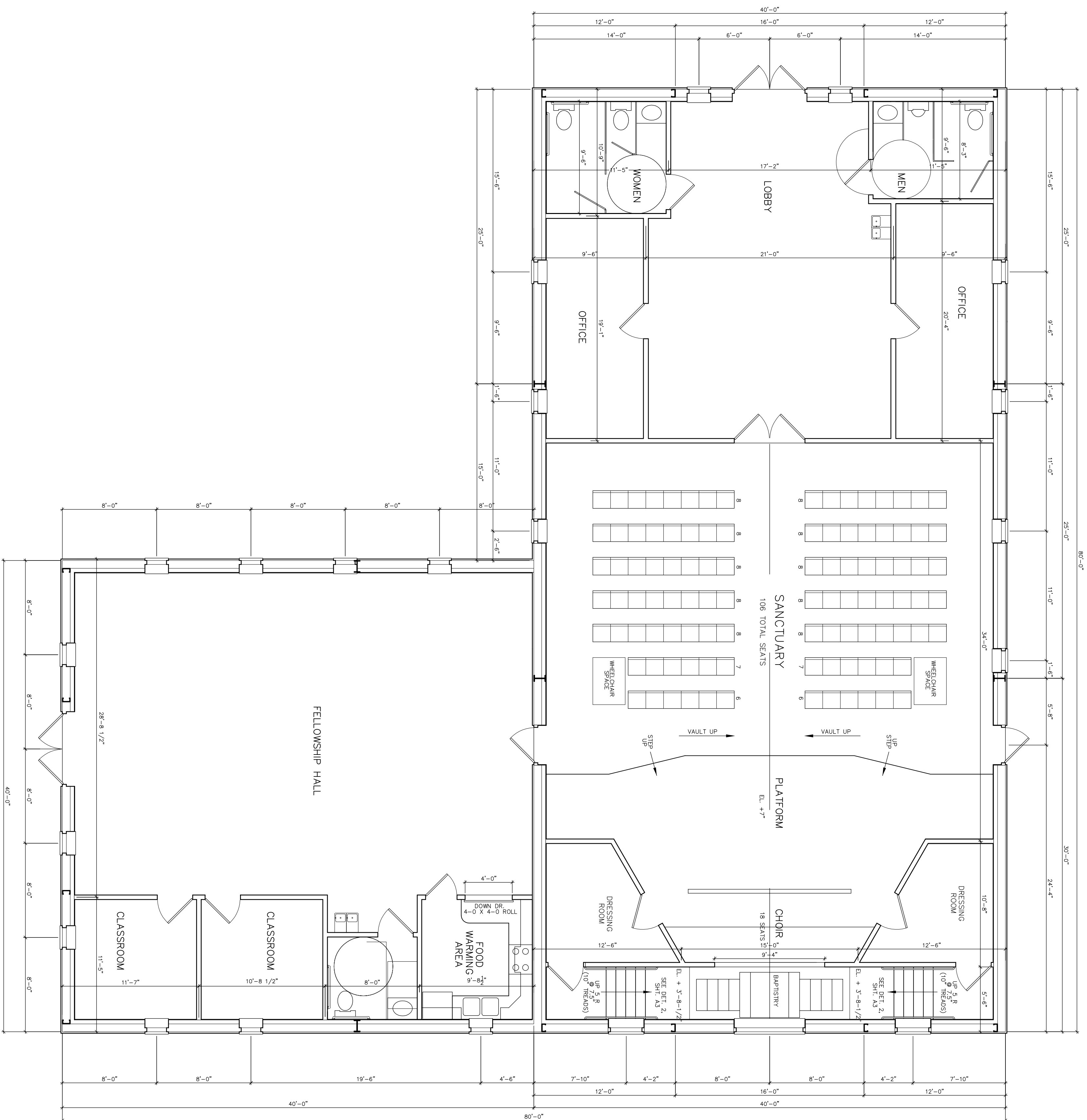
1 FLOORPLAN SCALE: 3/16" = 1'-0"
